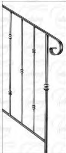
H 450 mm N 053.01 40x8 N 054.01 50x10 H 330 x L 100 mm N 056 40x8 H 330 x L 135 mm N 057 50x10 H 400 x L 180 mm N 056.01 40x8 N 057.01 50x10
